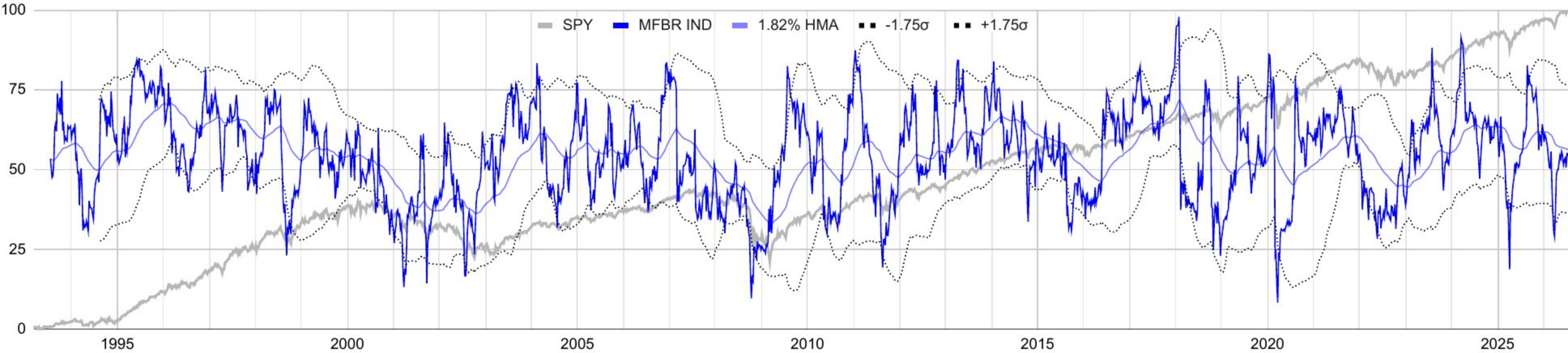
Z-Score
